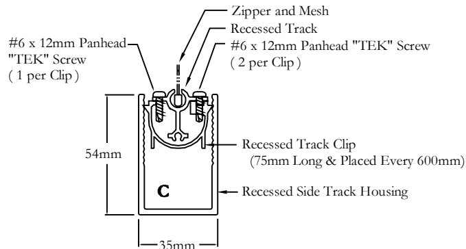
CROSS SECTIONAL VIEW OF THE FULLY ASSEMBLED RECESSED SIDE TRACK (V3)
