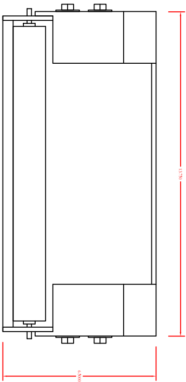
SIDE VIEW OF THE SUPPORT CARRIAGE
