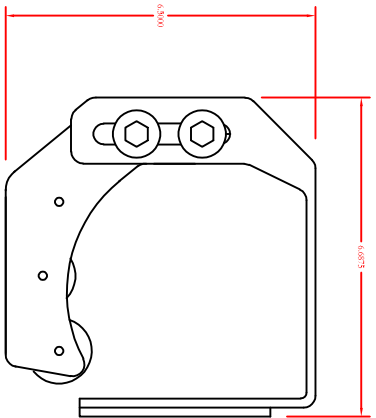
END VIEW OF THE SUPPORT CARRIAGE
