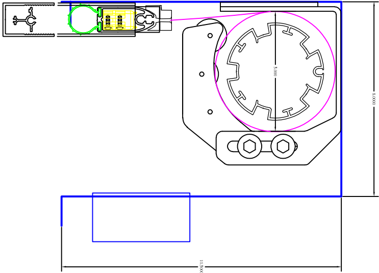
PLACEMENT OF 4" ROLLER, AND SUPPORT CARRIAGE IN A CAVITY
